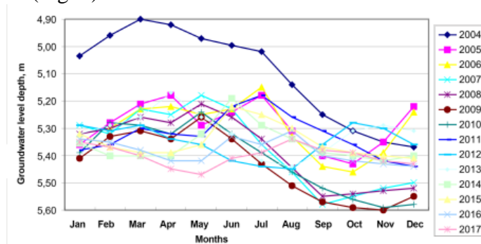
Fig. 1 – groundwater level changing in the well on the Kontorskaya street
