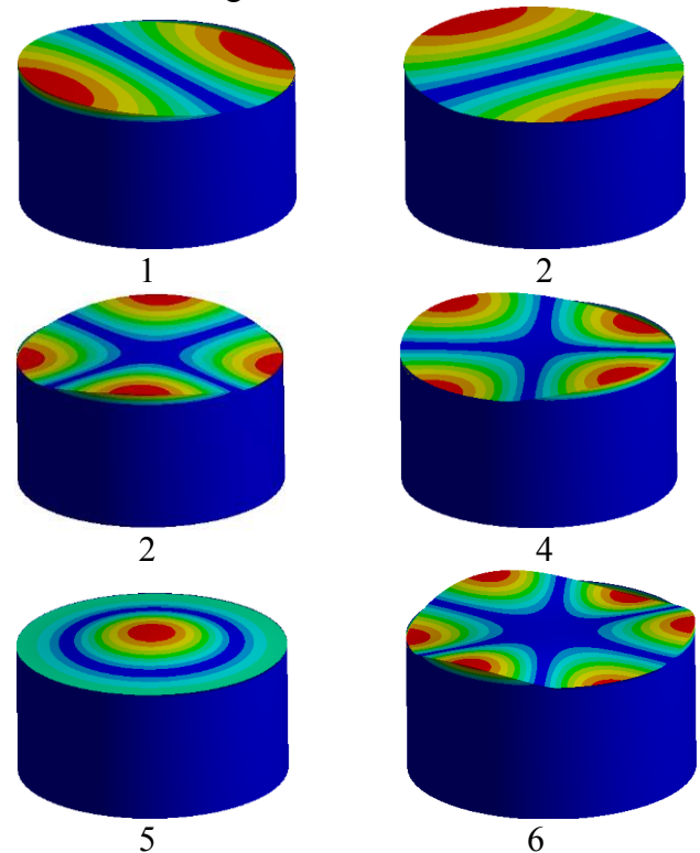
Fig. 4. The free surface sloshing modes
