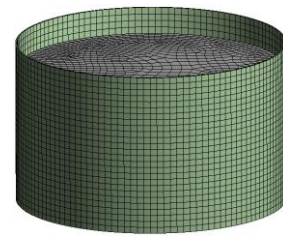
Fig. 3. Finite element grid for acoustic calculation
