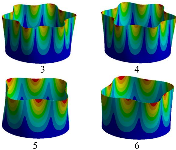
Fig.2. Oscillations modes of the unfilled shell The eigenfrequencies of the unfilled shell have been given for different materials in Table 1.
