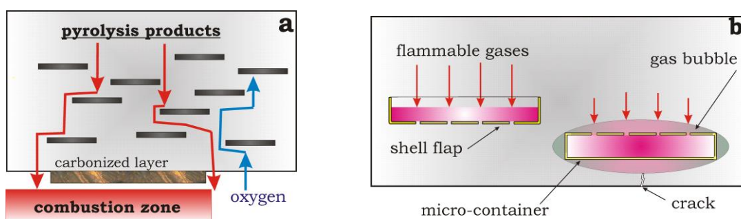
Fig. 1. Scheme of the barrier (a) and the proposed mechanism (b) of flame retardation
