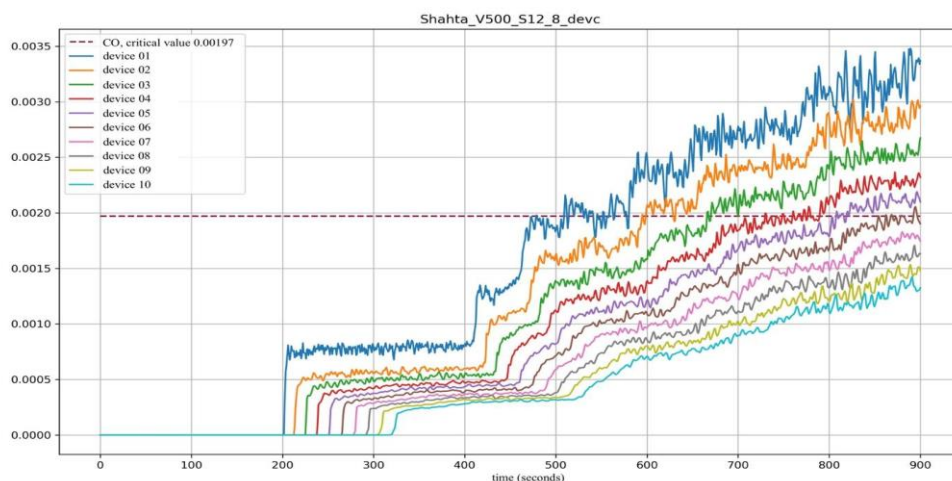
Figure 2: Dynamics of CO at the site 0 to 95 m from the source of the fire in the working with an area of 12.8 m 2 and airflow of 500 m 3 /min as evidenced by the sensors located at the top of the vault. The dashed line indicates the CO level that exceeds the MPC at the workplace
