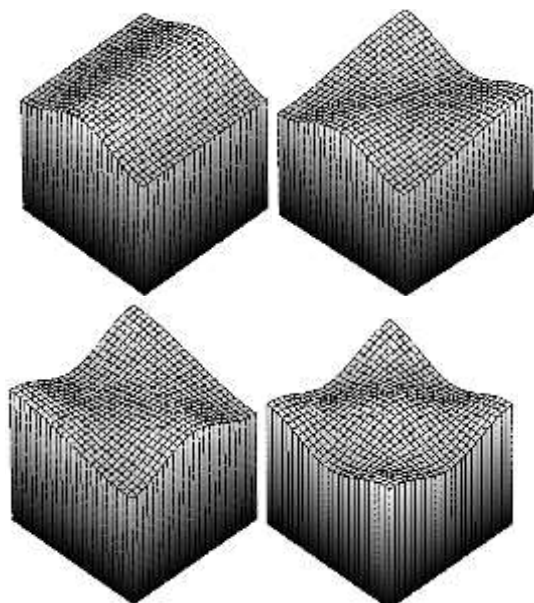
Fig.2. Modes of free surface vibrations in the prismatic tank
