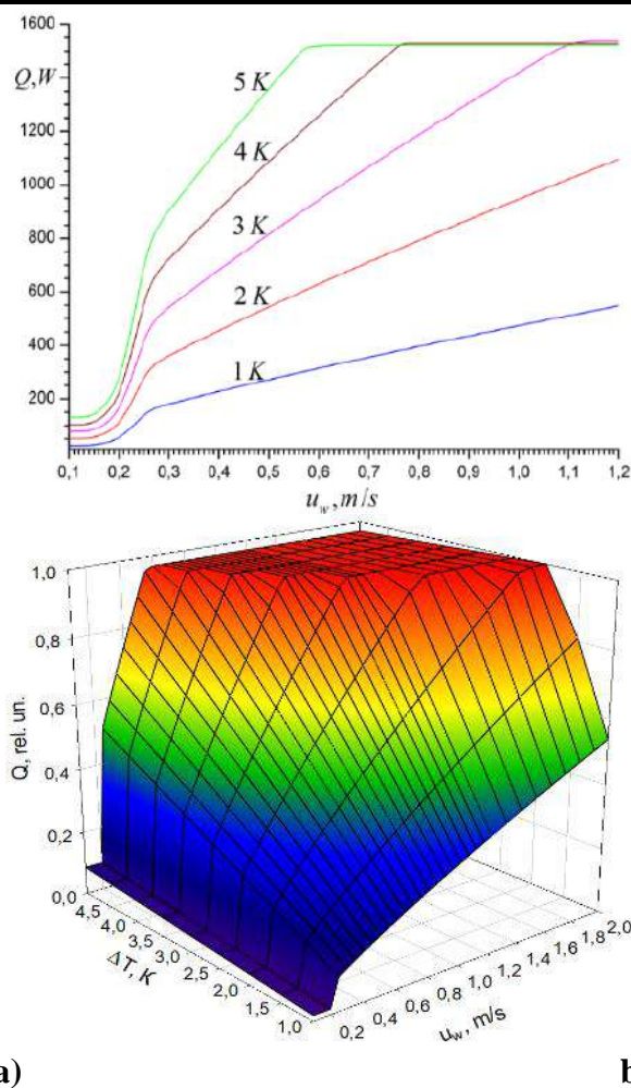
Fig. 1. The dependence of the amount of heat Q , which is diverted from the system when coolant flows through it at T=293 K, by water flow rate u_w for different temperature gradients \Delta T=1,2,3,4,5 K.
