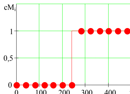
Fig. 6. Dynamics of output signal cM_i of the learning fire detector under examined conditions
