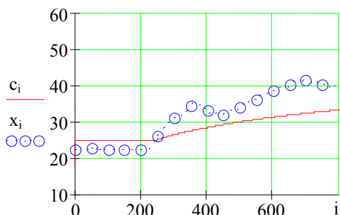
Fig. 5. Dynamics of the learning threshold and the mean temperature of medium in the chamber over the initial interval of data recording
