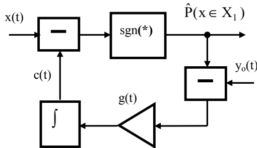
Fig. 1. Block diagram of the learning fire detector, at whose output the current estimation \hat{P}(x \in X_1) of probability P(x \in X_1) of the existence of a fire site is formed
