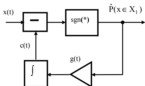
Fig. 2. Block diagram of the self-learning fire detector, at whose output the current estimation \hat{P}(x \in X_1) of probability P(x \in X_1) of the existence of a fire site on the object is formed
