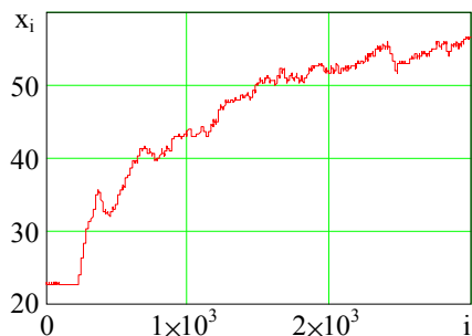
Fig. 4. Dynamics of the mean temperature of medium in the simulating chamber over the assigned registration interval (300 s)
