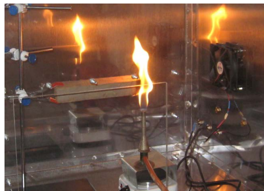
Fig. 3. Exterior view of the simulating chamber with openings
